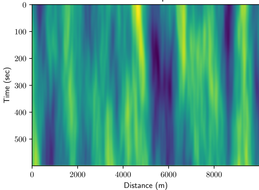
Wind Map
